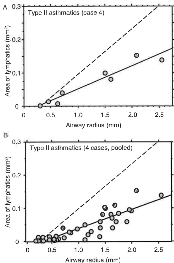
Fig. 5 The distribution of airway lymphatics in Type II asthmatics. A: The data of total areas of lymphatics around each airway of Type II asthmatics (Case 4), 8 airways in total, were plotted ( r = 0.928 , p < 0.001 ). In comparison with the regression line of 5 control lungs, revealed as a broken line, the lymphatic distribution in the airway walls of this case is decreased. B: The pooled data of the lymphatics around each airway of 4 cases of Type II asthmatics, 42 airways in total, were plotted. Although the data are dispersed among the cases, there is again a positive correlation between them ( r = 0.768 , p < 0.001 ). The lymphatic distribution around airways of these patients is decreased in comparison with the regression line in controls (a broken line).
